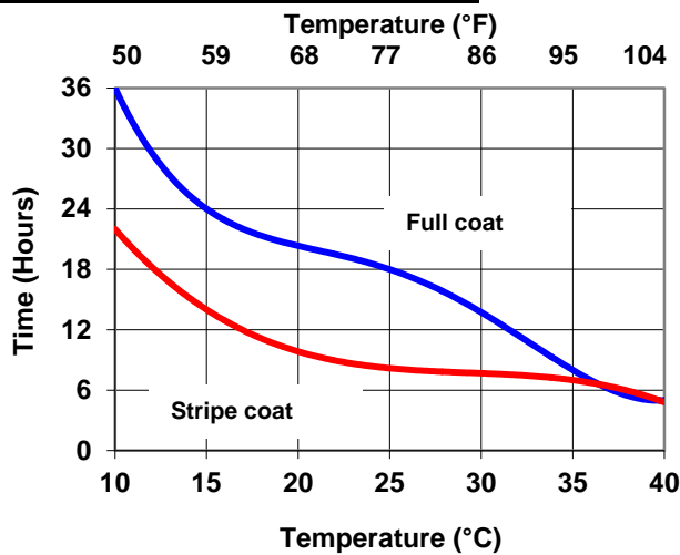
Interline 925: Minimum Overcoating
