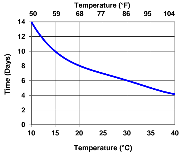
Interline 925: Curing Time
