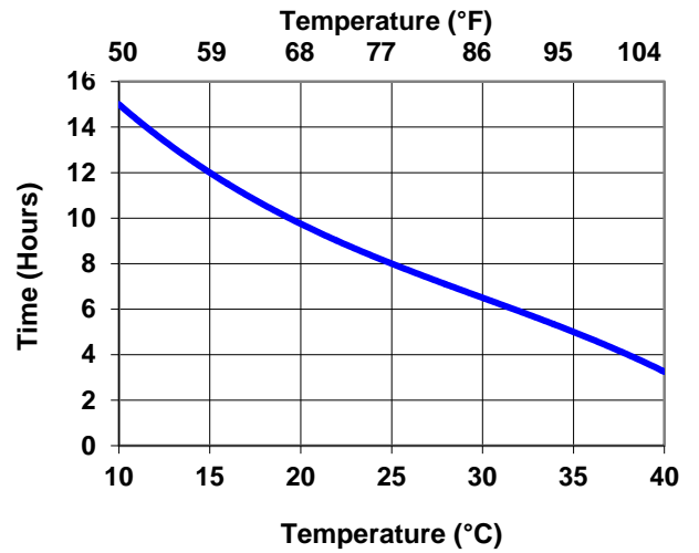
Interline 925: Touch Dry
