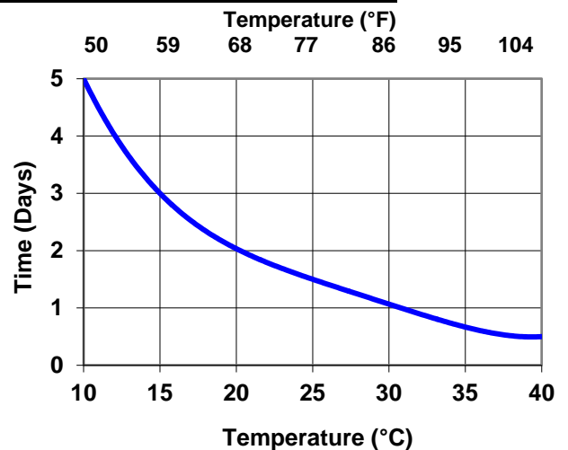
Interline 925: Maximum Overcoating
