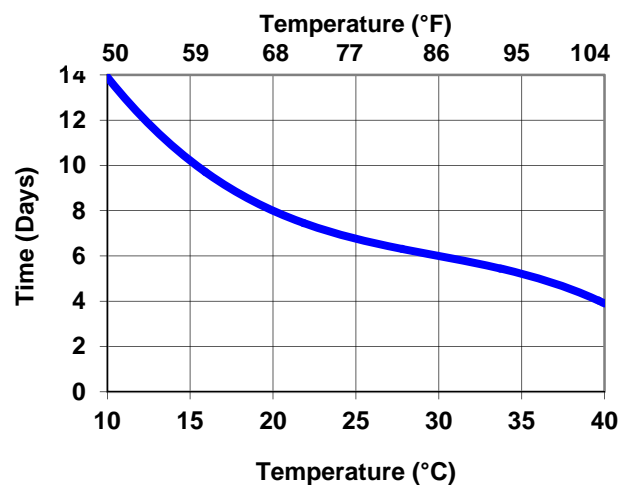
Interline 975: Curing Time
