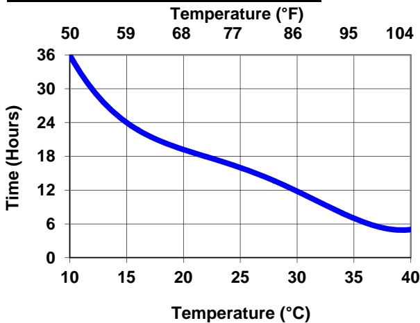
Interline 975: Minimum Overcoating
