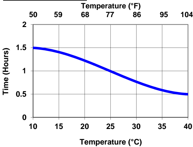
Interline 975: Pot Life
