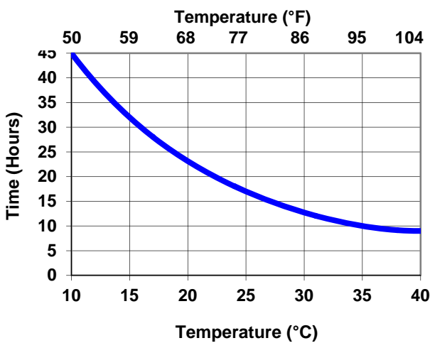
Interline 975: Hard Dry
