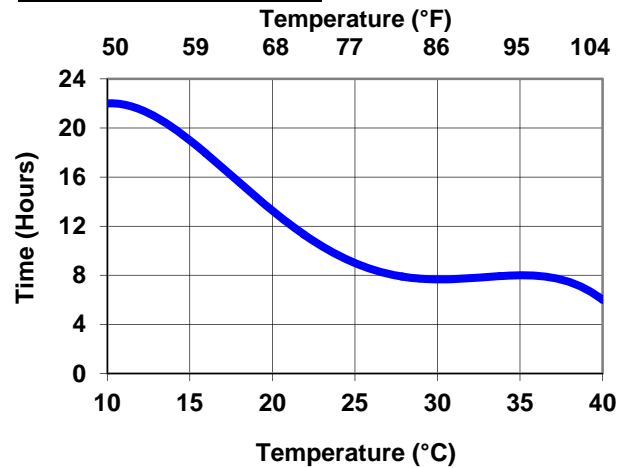
Interline 975: Touch Dry
