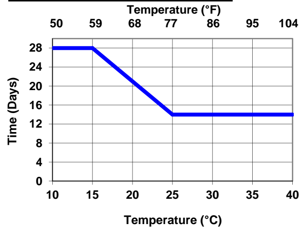
Interline 975: Maximum Overcoating
