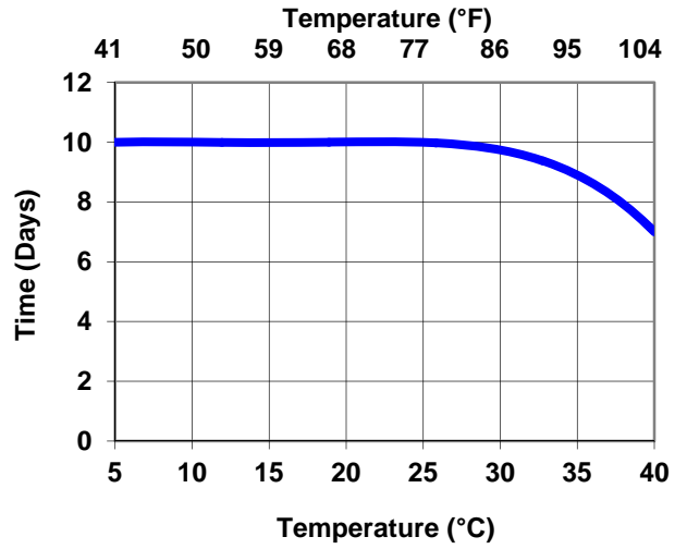
Interline 344: Maximum Overcoating
