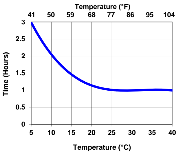
Interline 344: Hard Dry
