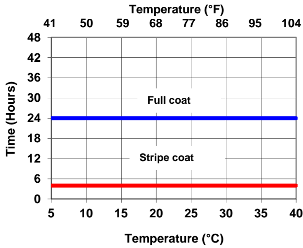
Interline 344: Minimum Overcoating
