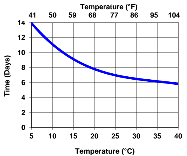
Interline 344: Curing Time following minor repairs
