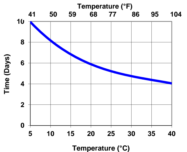
Interline 104: Maximum Overcoating
