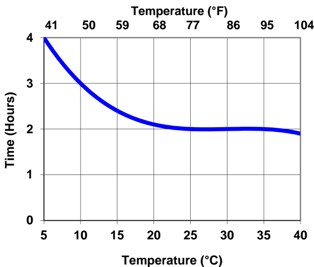
Interline 104: Minimum Overcoating
