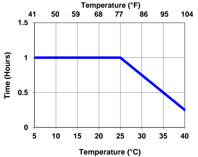
Interline 104: Curing Time following minor repairs
