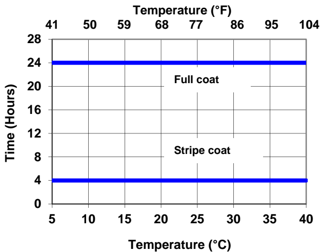
Interline 104: Minimum Overcoating
