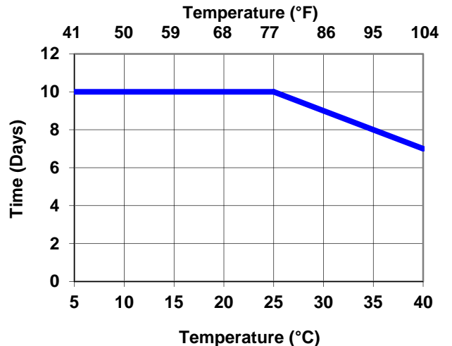
Interline 104: Maximum Overcoating
