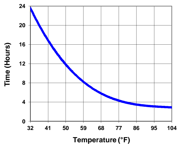
Interline 783: Minimum Overcoating
