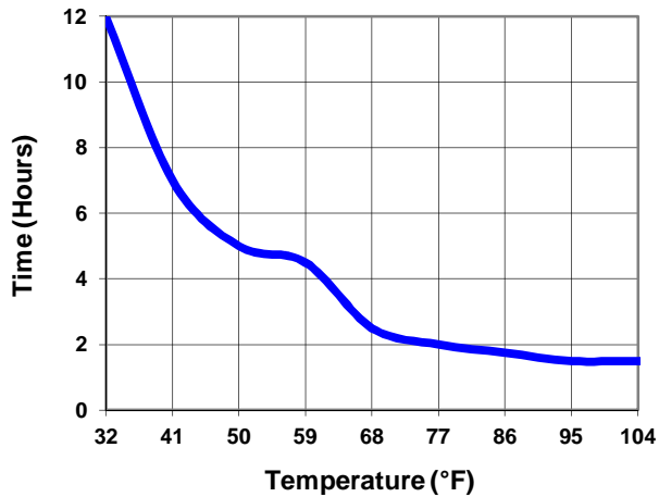
Interline 783: Touch Dry
