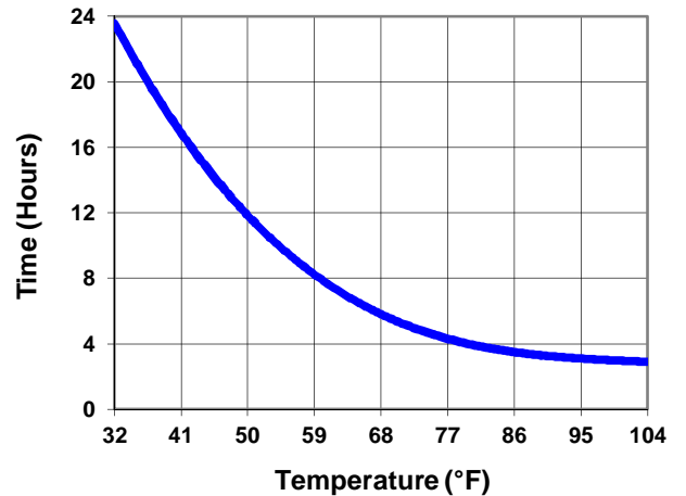
Interline 783: Hard Dry
