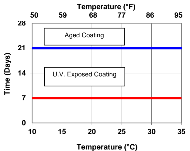
Interline 624: Maximum Overcoating Interval
