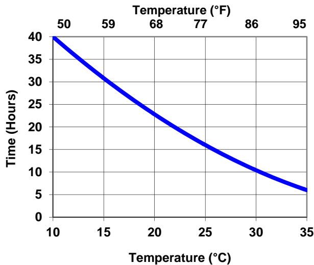
Interline 624: Minimum Overcoating Interval
