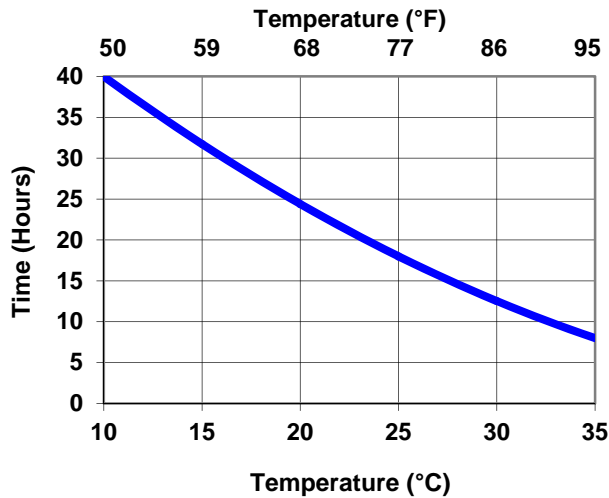
Interline 624: Minimum Overcoating Interval
