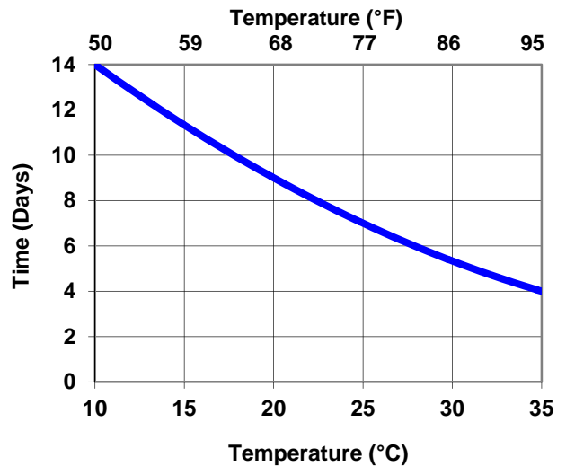
Interline 624: Maximum Overcoating Interval
