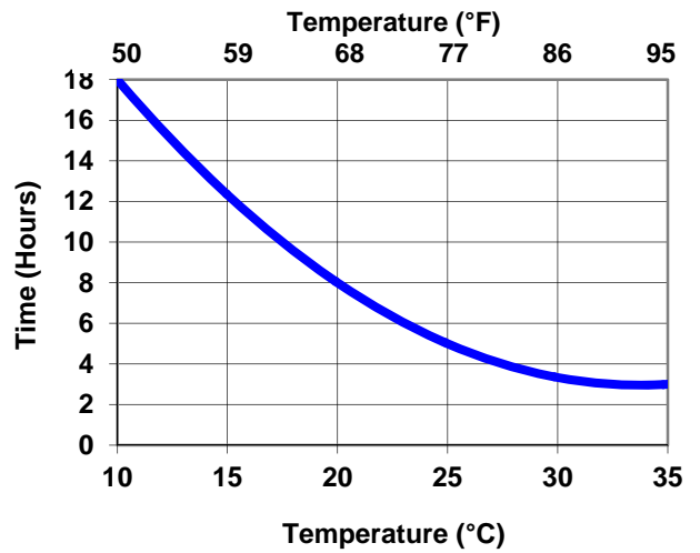
Interline 624: Touch Dry
