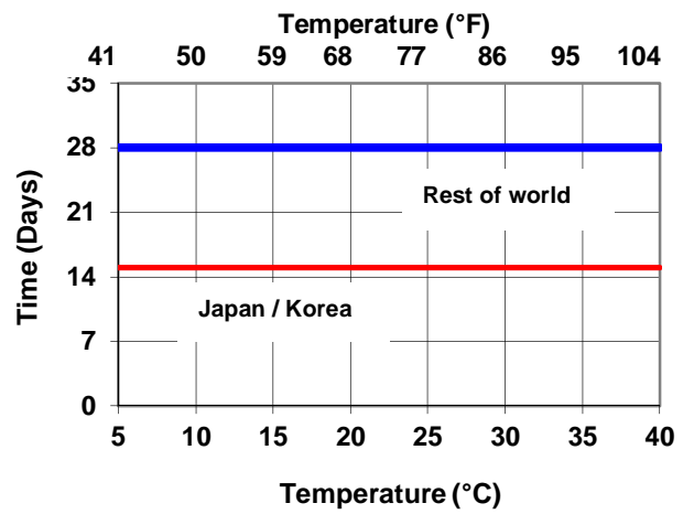
Intergard 403: Maximum Overcoating
