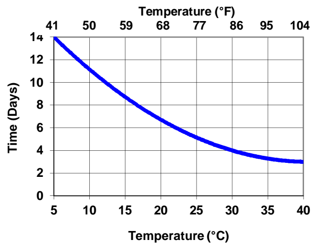
Intergard 403: Maximum Overcoating
