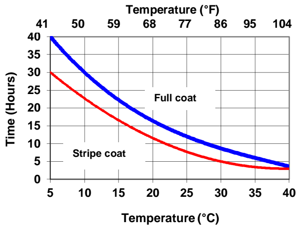
Intergard 403: Minimum Overcoating
