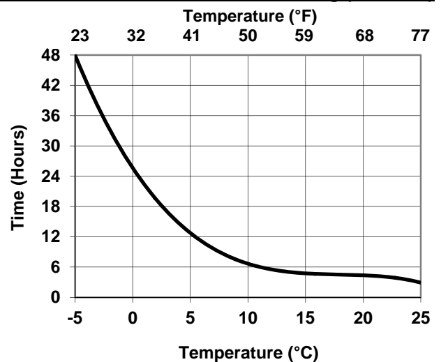
Interbond 201LT: Minimum Overcoating (Full coat)
