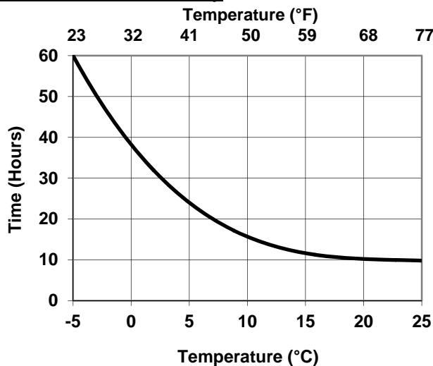
Interbond 201LT: Hard Dry
