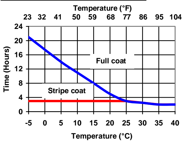
Intergard 7500: Minimum Overcoating
