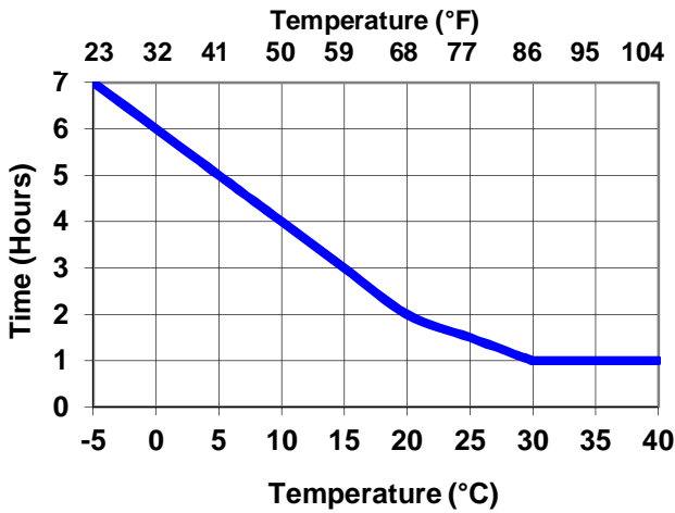
Intergard 7500: Pot Life
