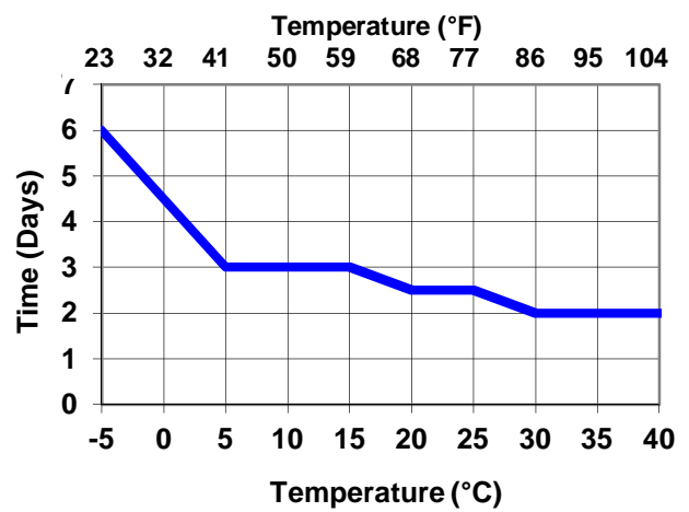
Intergard 7500: Time to Ballast
