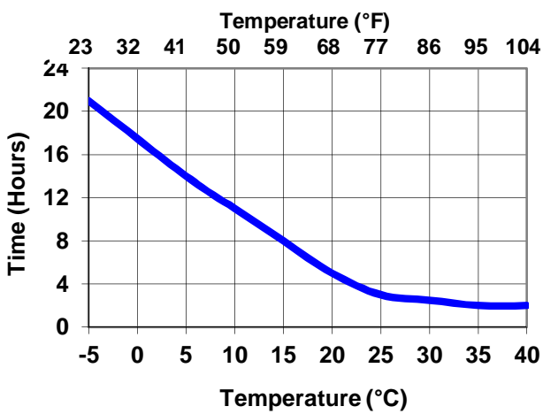
Intergard 7500: Hard Dry
