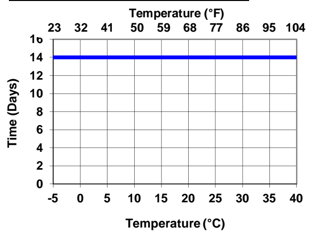
Intergard 7500: Maximum Overcoating
