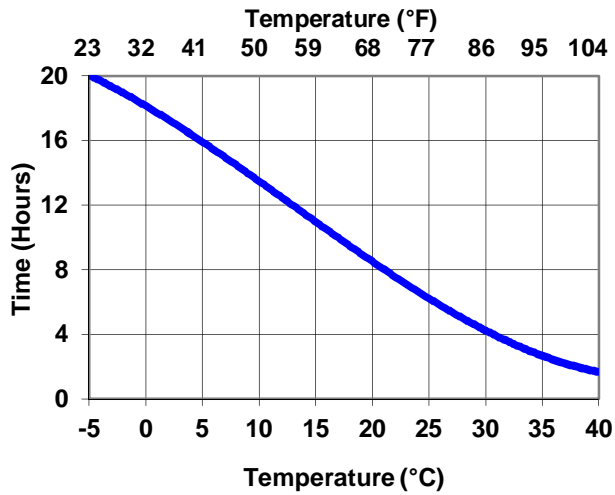
Intershield 300: Walk-On Time
