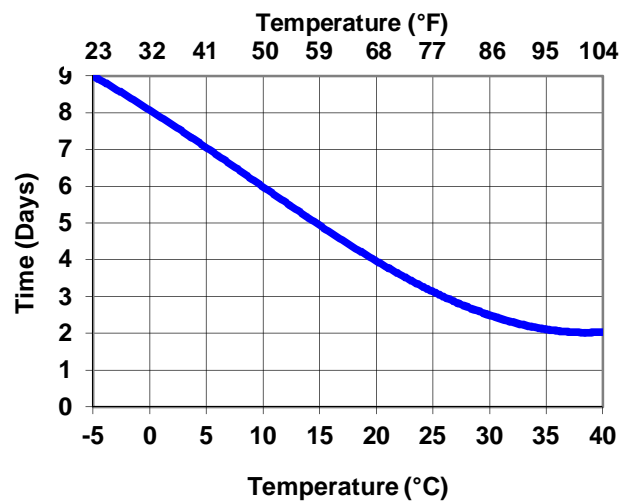
Intershield 300: Time to Ballast
