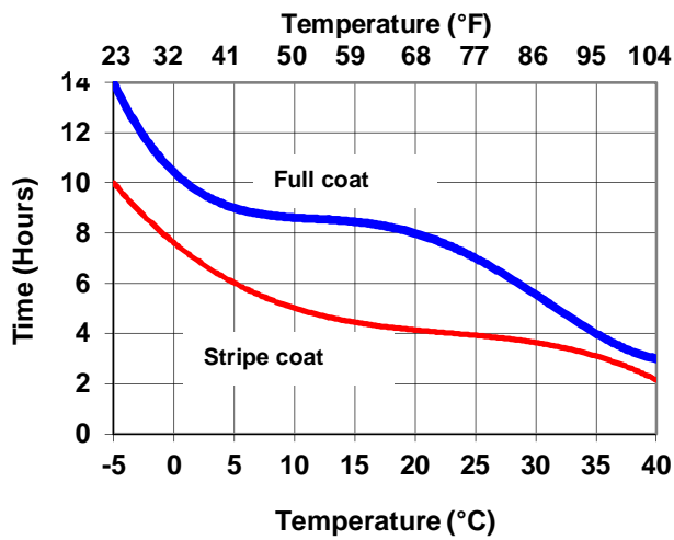
Intershield 300: Minimum Overcoating
