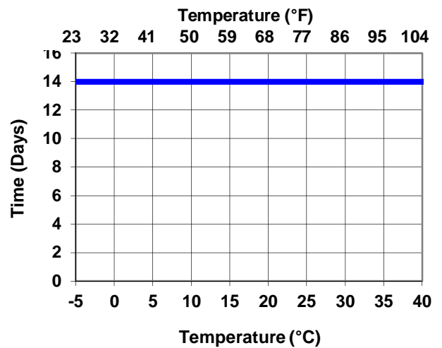
Intershield 300: Maximum Overcoating
