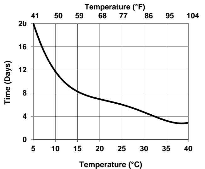
Interline 904: Maximum Overcoating
