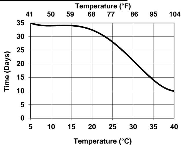
Interline 904: Maximum Overcoating
