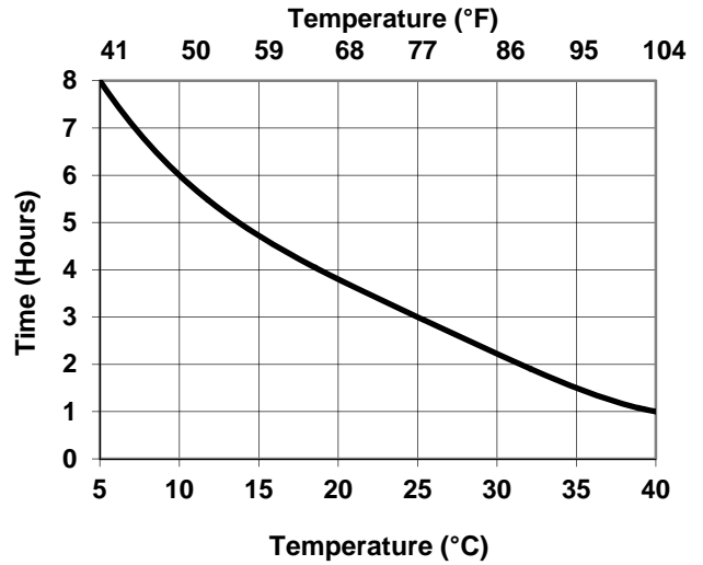
Interline 904: Curing Time
