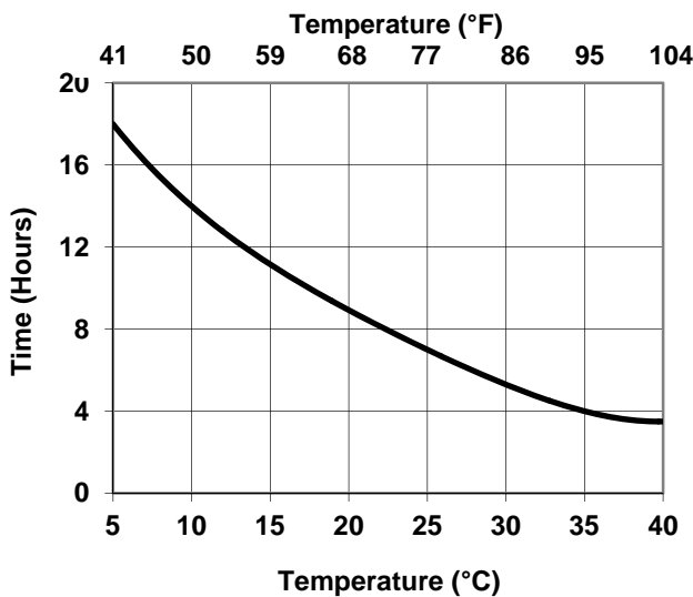
Interline 904: Minimum Overcoating
