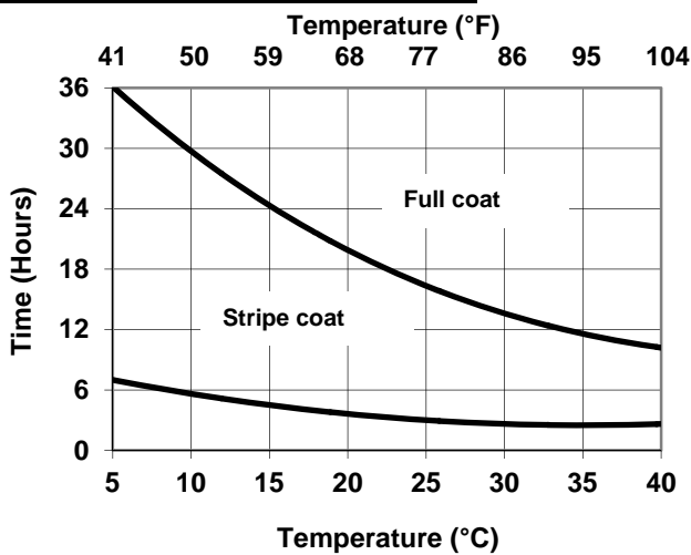
Interline 904: Minimum Overcoating
