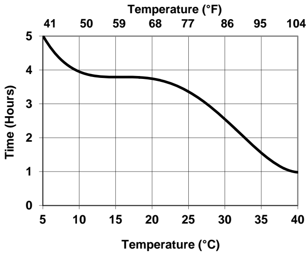
Interline 904: Hard Dry
